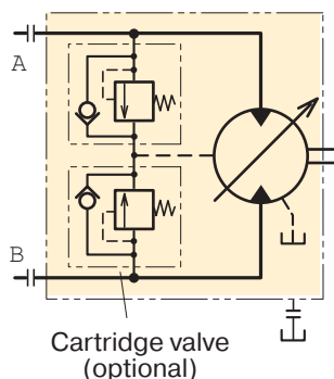
Hydraulic schematic
