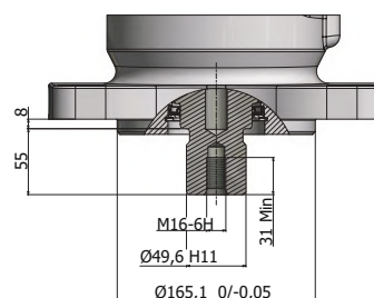
Shaft code D, -220
