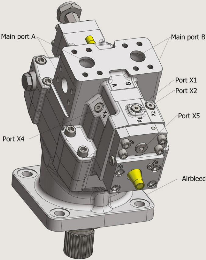
Port locations – V16- with AC compensator.
