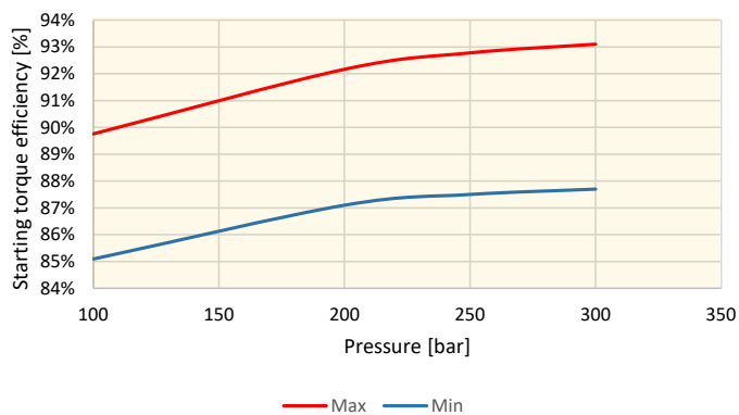
V16-270 limited displacement = 220 cc/rev
