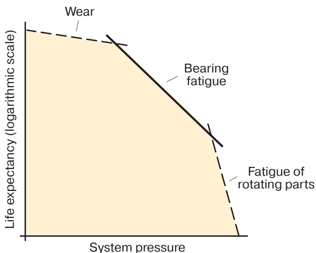
Hydraulic motor life versus system pressure.
