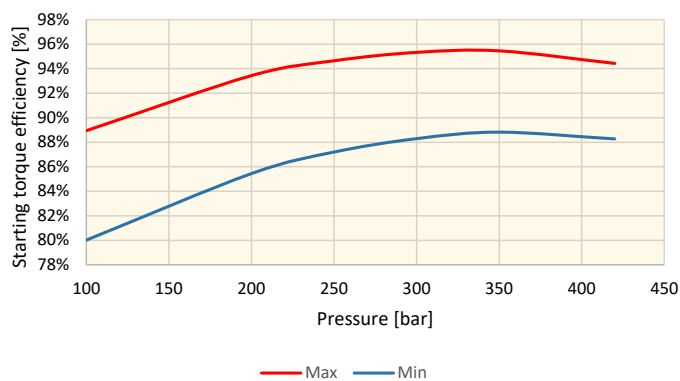
V16-220 limited displacement = 180 cc/rev
