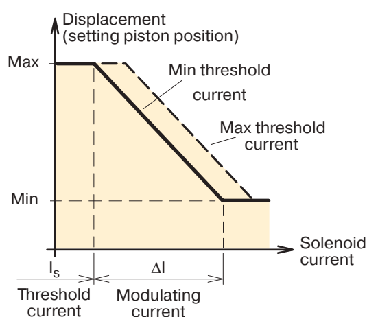
EP diagram (displacement vs. solenoid current).
