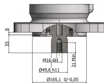
Shaft code Z, -270
